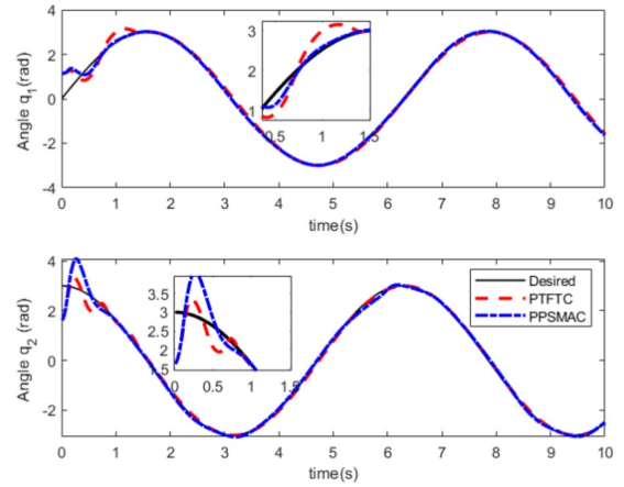
Fig. 14. Angle tracking curve under different controllers.
