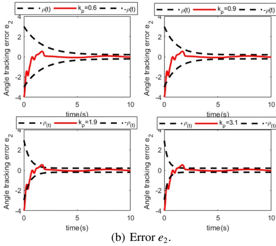
Fig. 3. Angle tracking error under different convergence rates.
