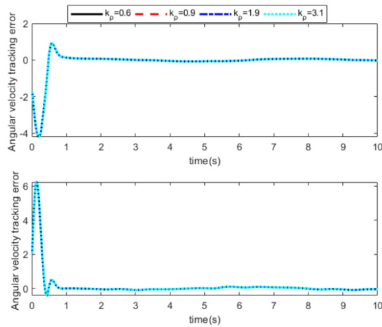
Fig. 8. Angular velocity tracking error under different convergence rates.
