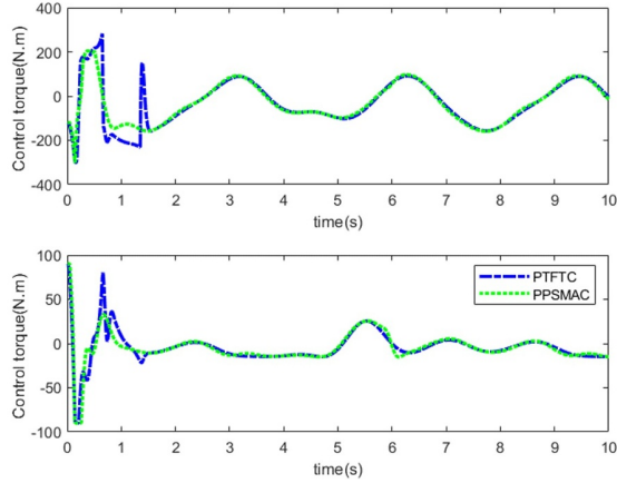
Fig. 17. Actual control input under different controllers.
