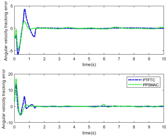
Fig. 16. Angular velocity tracking error under different controllers.
