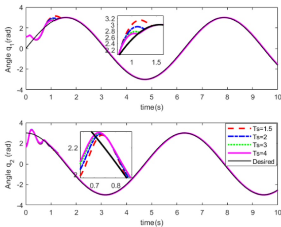
Fig. 10. Angle tracking curve under different predefined times.
