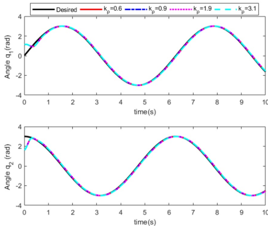
Fig. 6. Angle tracking curve under different convergence rates.
