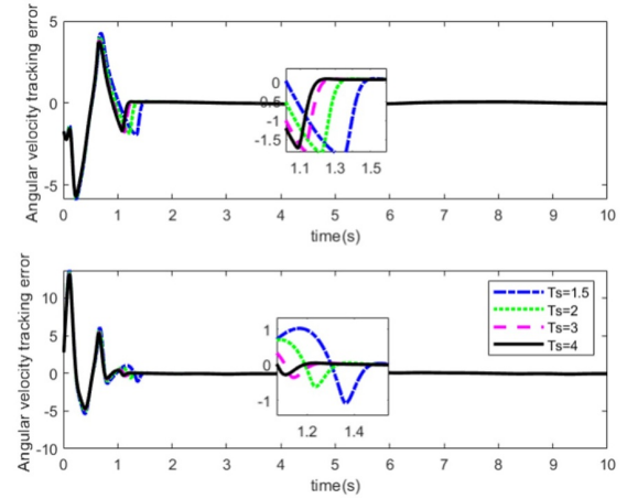
Fig. 12. Angular velocity tracking error under different PCT.
