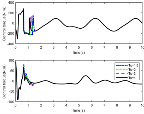
Fig. 13. Actual control input under different PCT.
