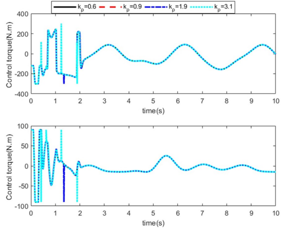
Fig. 5. Actual control input under different convergence rates.
