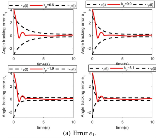
Fig. 2. Angle tracking curve under different convergence rates.
