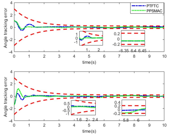
Fig. 15. Angle tracking error under different controllers.
