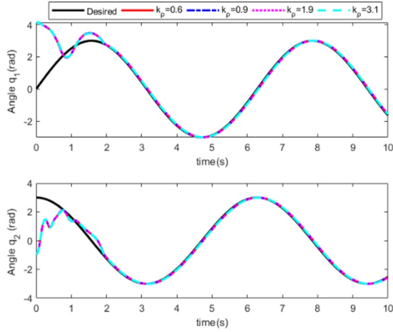
Fig. 2. Angle tracking curve under different convergence rates.
