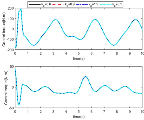
Fig. 9. Actual control input under different convergence rates.
