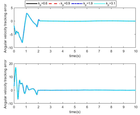
Fig. 4. Angular velocity tracking error under different convergence rates.
