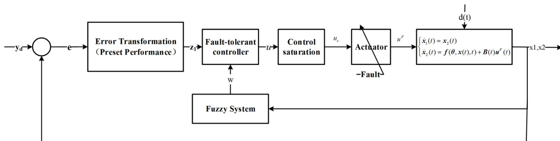
Fig. 1. Structure diagram of adaptive fuzzy fault-tolerant control.
