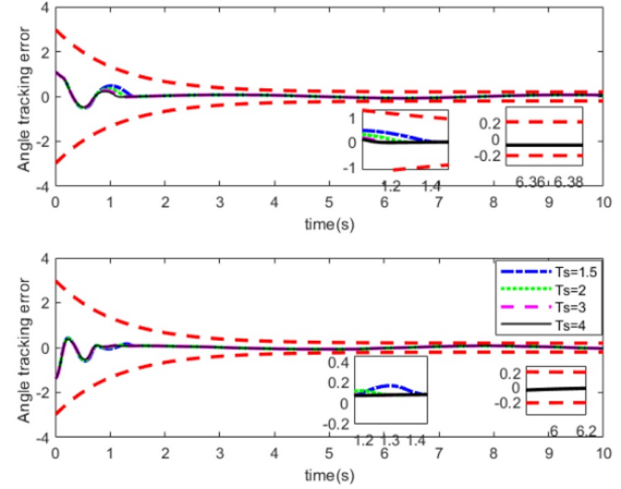
Fig. 11. Angle tracking error under different PCT.
